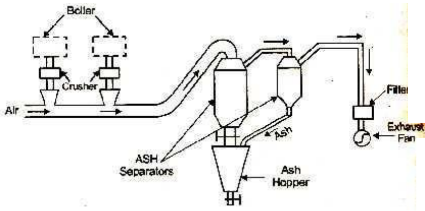
Figure: Pneumatic system
