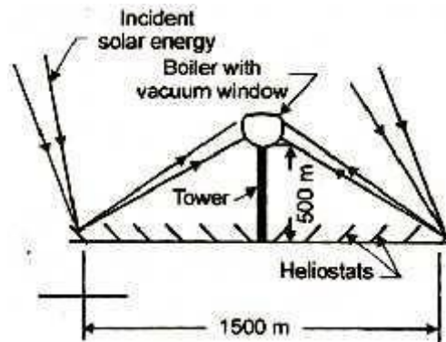
Figure: Tower concept for power generation.
