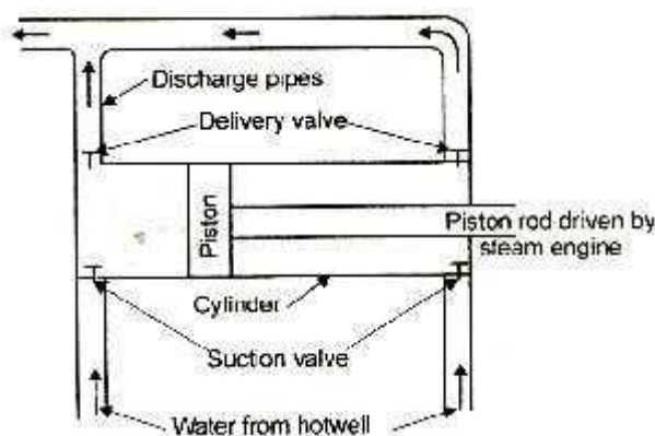
Figure: Feed pump (reciprocating type).
