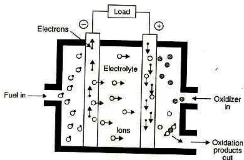
Figure: Schematic of a fuel cell.
