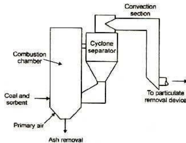
Figure: Circulating bed combustor.
