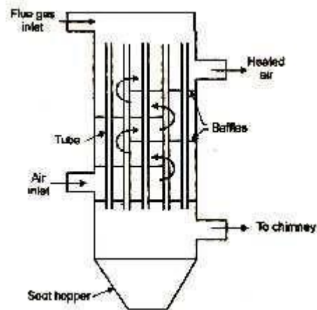
Figure: Air pre-heater
