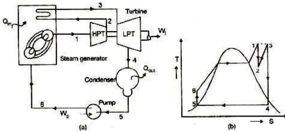
Figure: Schematic diagram and T-S diagram of Rankine cycle with reheat.
