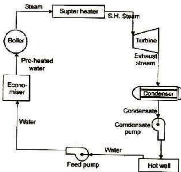
Figure: Water and Steam circuit
