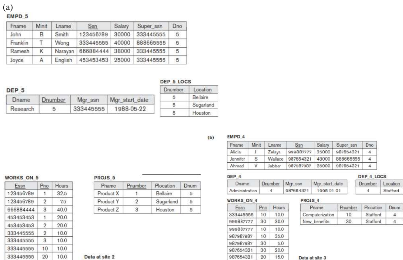
Figure. Allocation of fragments to sites. (a) Relation fragments at site 2 corresponding to department 5. (b) Relation fragments at site 3 corresponding to department 4.
