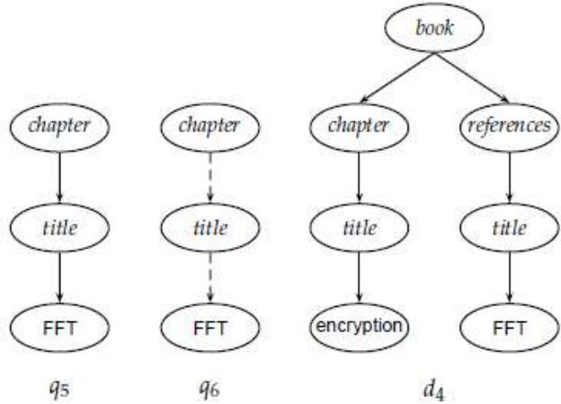
Figure . A structural mismatch between two queries and a document.
