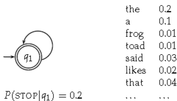
Figure: A one-state finite automaton that acts as a unigram language model. We show a partial specification of the state emission probabilities.
