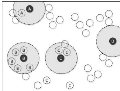
Fig. Example of overlapping clustering using Parzen windows. The clusters for the black points (A, B, C, and D) are shown. The shaded circles indicate the windows used to determine cluster membership. The neighbors for each black point are shaded gray and labeled accordingly.
