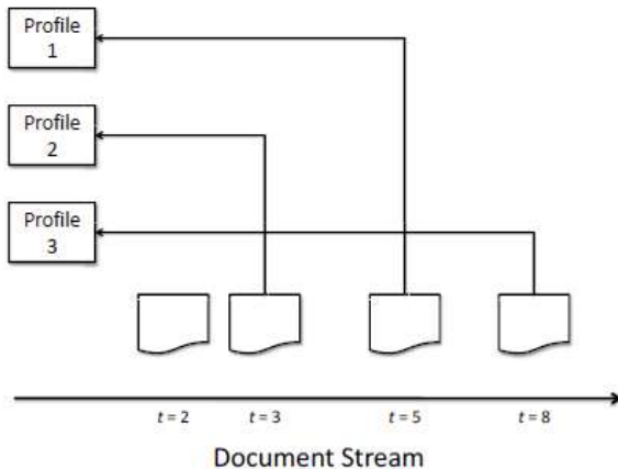
Fig. Example of a static filtering system. Documents arrive over time and are compared against each profile. Arrows from documents to profiles indicate the document matches the profile and is retrieved.
