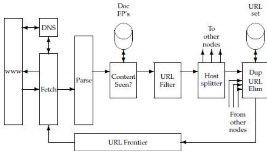
Figure . Distributing the basic crawl architecture.
